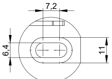
DETAIL A (4x) SCALE 1 : 1
